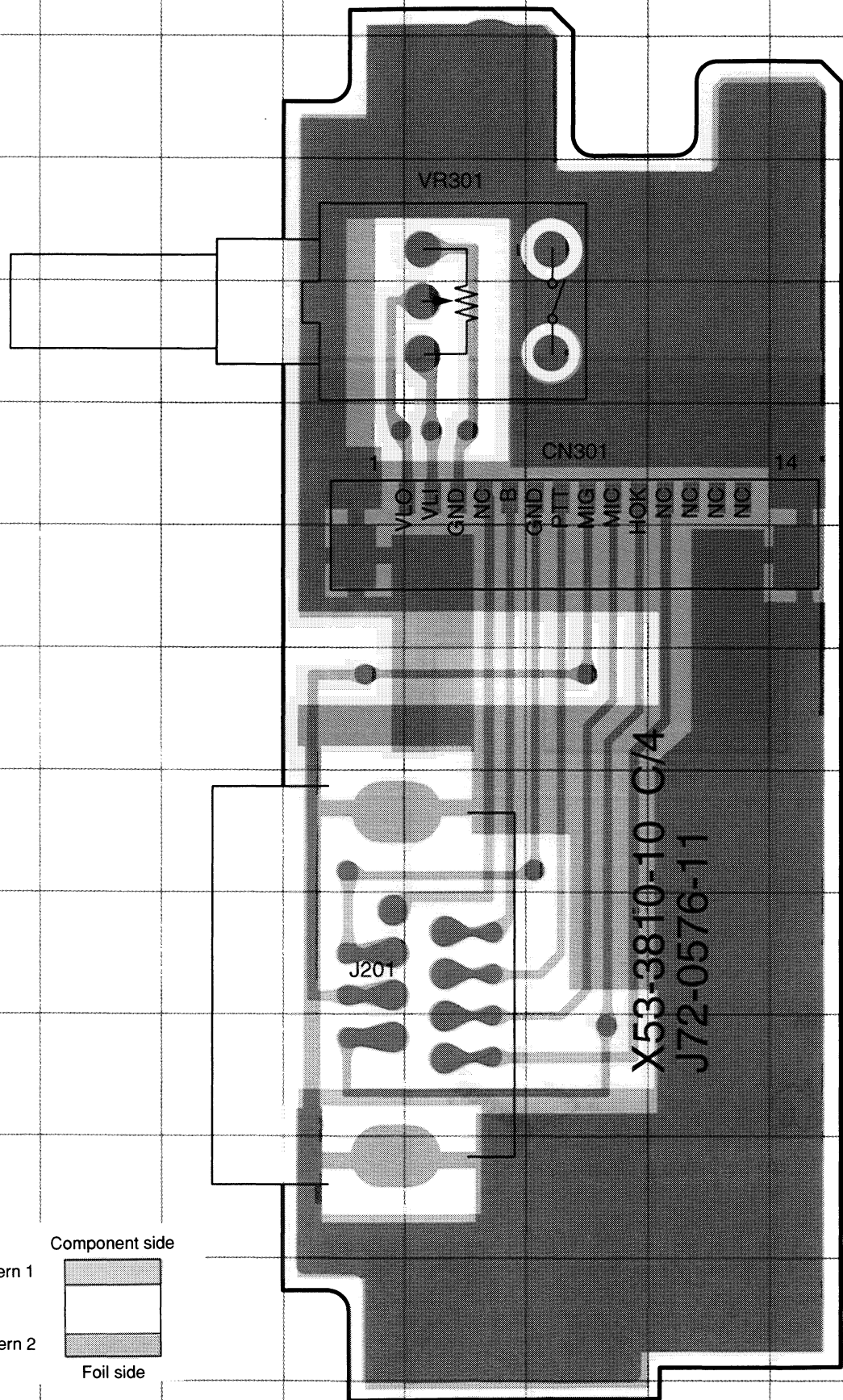
CONTROL UNIT (X53-3810-10) (C/4) Component side view
