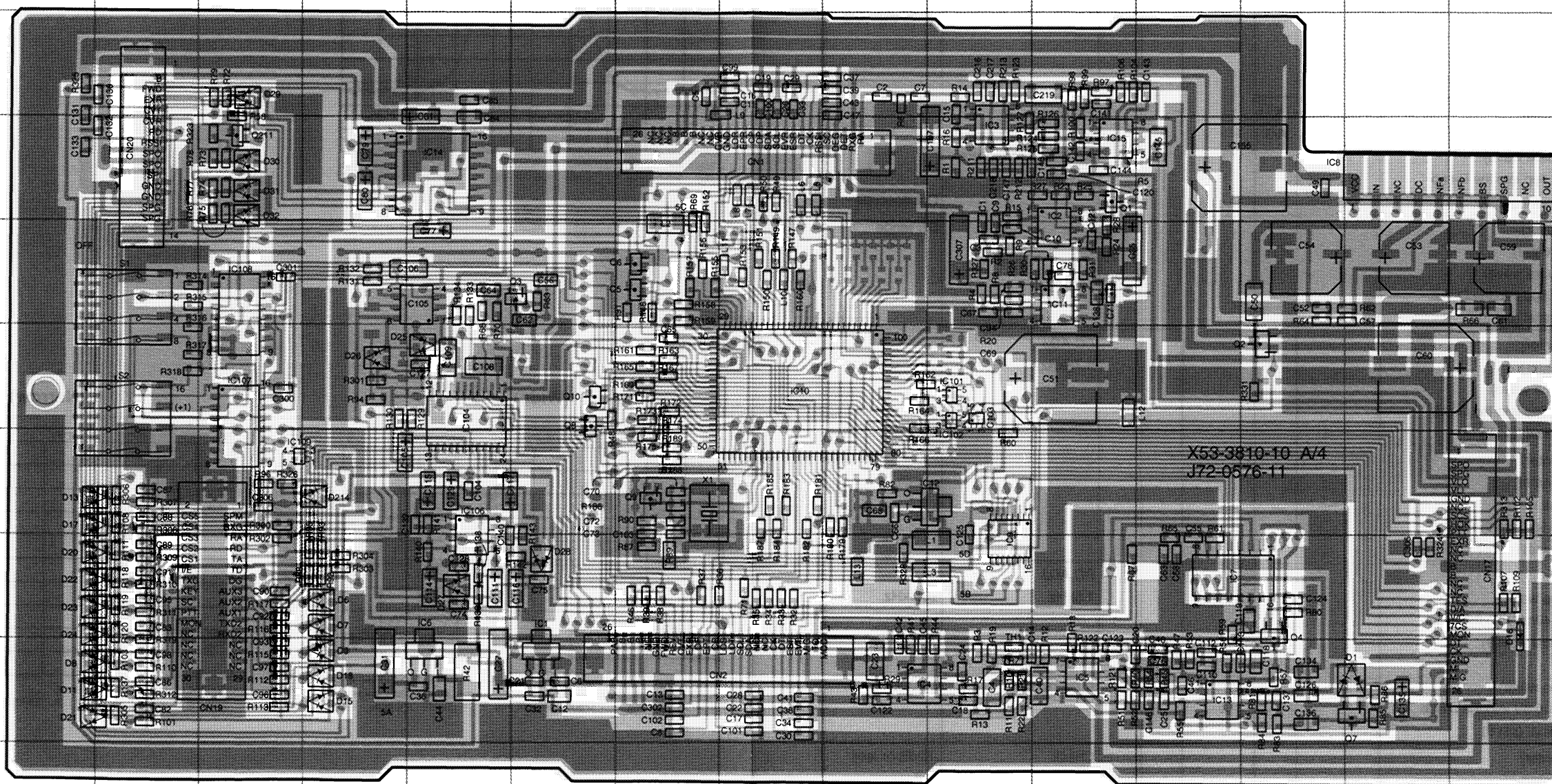
CONTROL UNIT (X53-3810-10) (A/4) Component side view
