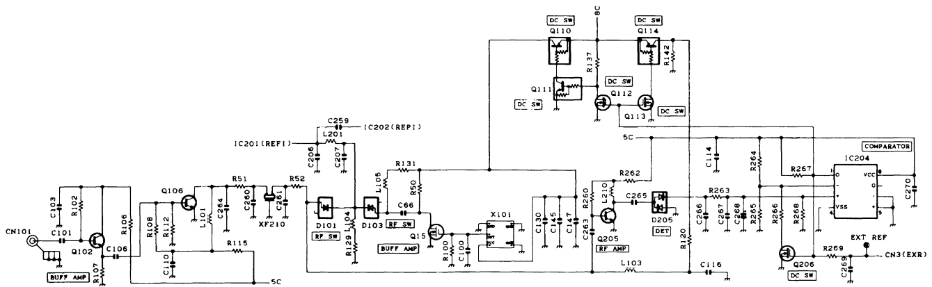
Fig.1 Internal/external reference circuit
