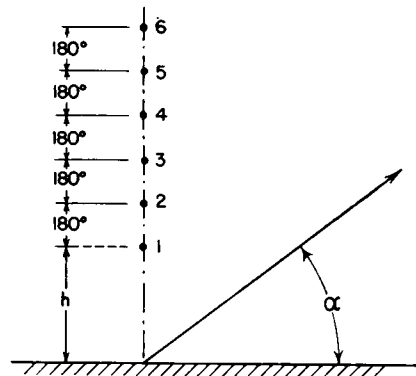
FIG. 3.37. Vertical stack of equal-current cophased dipoles.
