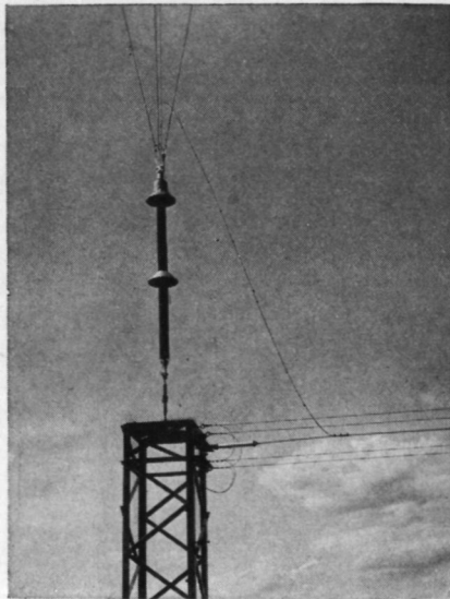
FIG. 1.41. Down-lead insulator and the end of the six-wire unbalanced unmatched feeder for the antenna of Fig. 1.5.
