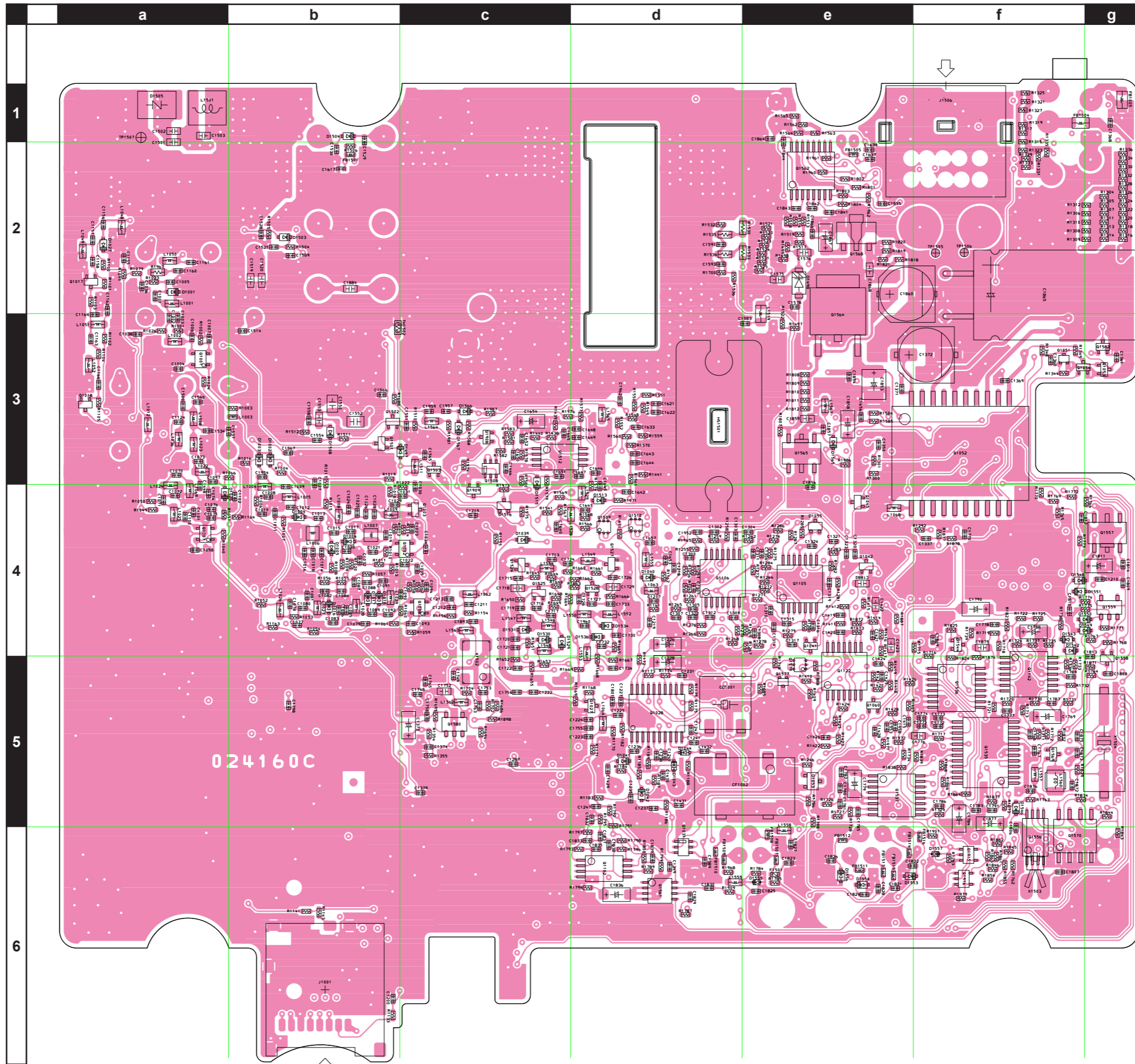
MAIN-3
