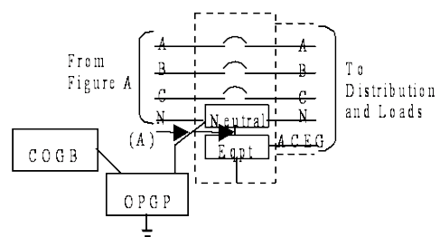
D. Service Disconnect Equipment Grounded AC Service Water Pipe or Driven Ground Electrode
