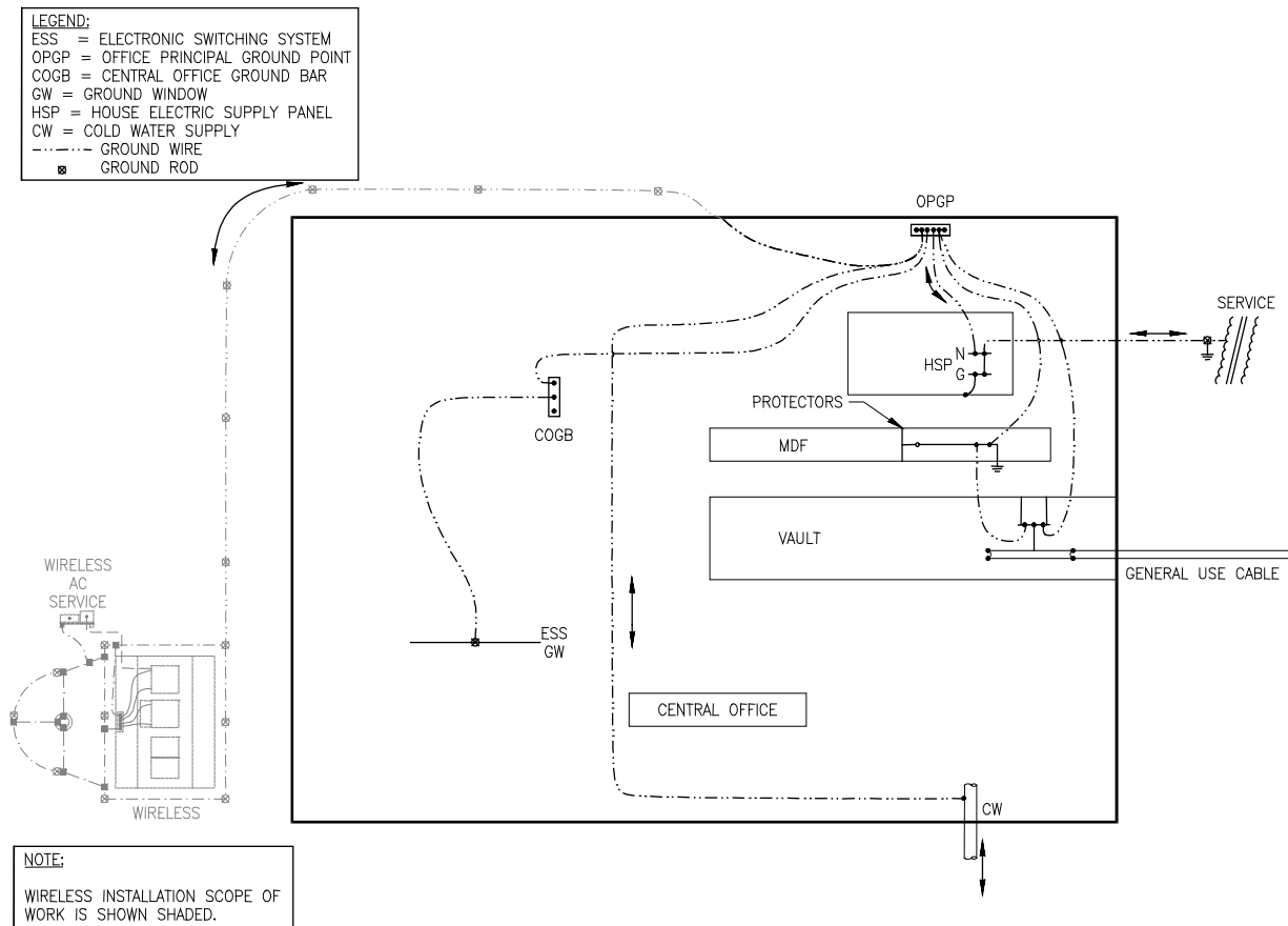
Figure 7-23: Grounding Interface Between the Ground Electrode Field of a Wireless Site and a CenturyLink CO that only has the Power Company MGN as a Ground Electrode Field
