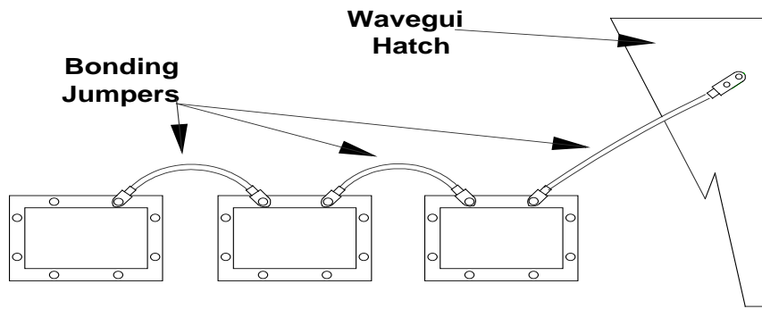
Bonding Outdoor Waveguide Flanges to Waveguide Hatch (Typical)
