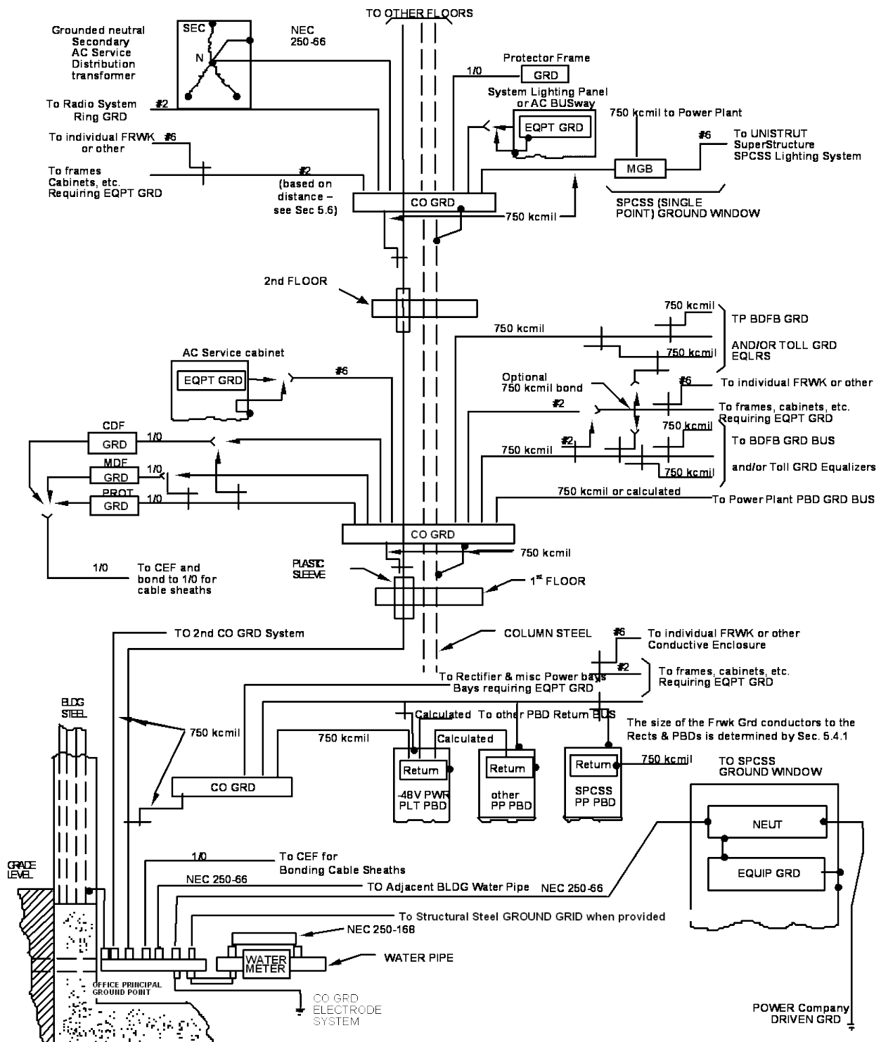
Figure 3-7: Typical Equipment Connected to a CO GRD System
