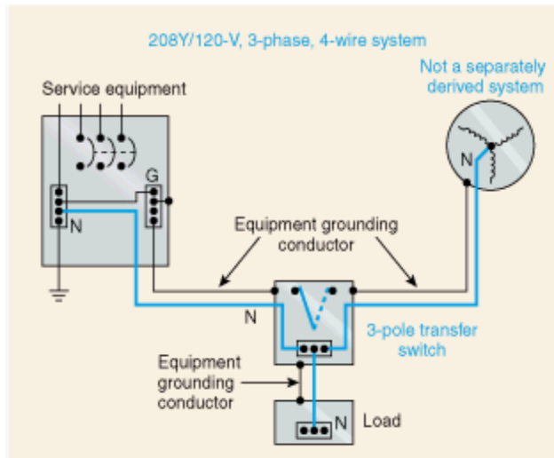
Figure 4-1: Typical Engine-Alternator that is Not Separately-Derived
