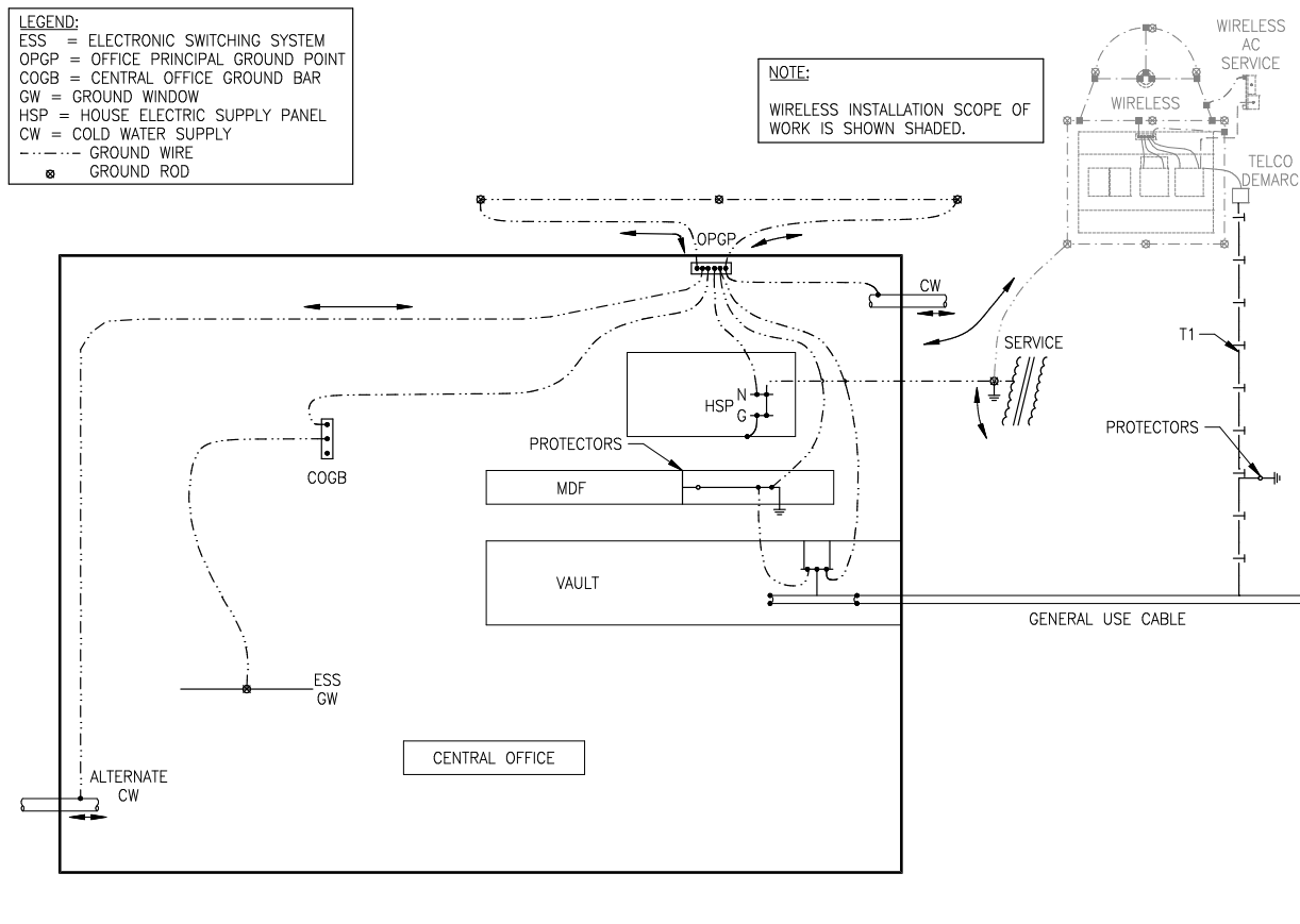
Figure 7-22: Grounding Interface Between the Ground Electrode Field of a Wireless Site and a CenturyLink CO Using a Deep Driven Rod, Counterpoise, or Chemical Ground (Ground Well) System
