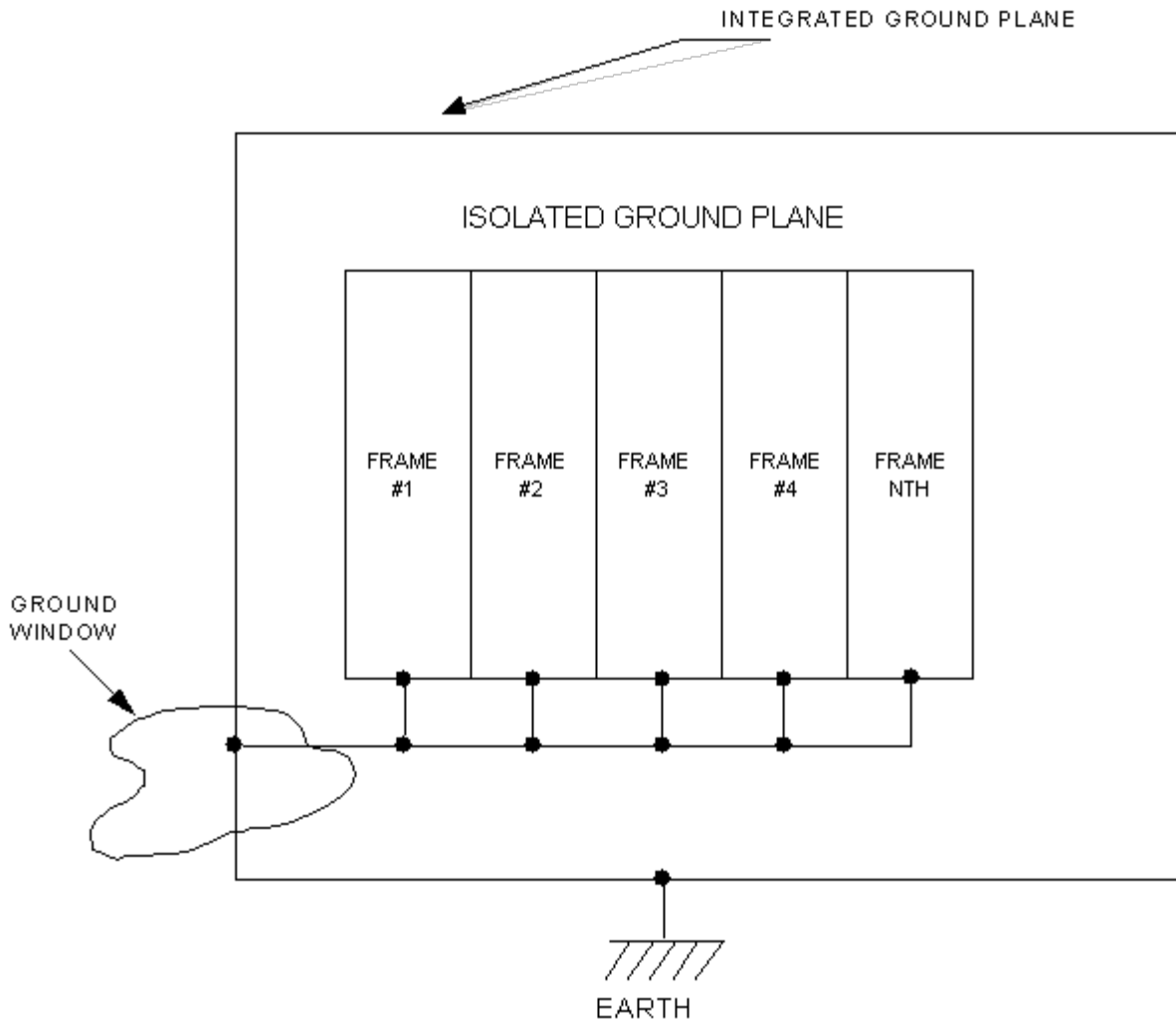
Figure 8-1: Simplified Isolated Ground Plane
