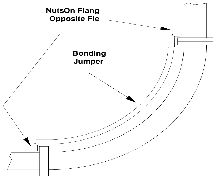
Flex Waveguide Bond (Typical)
