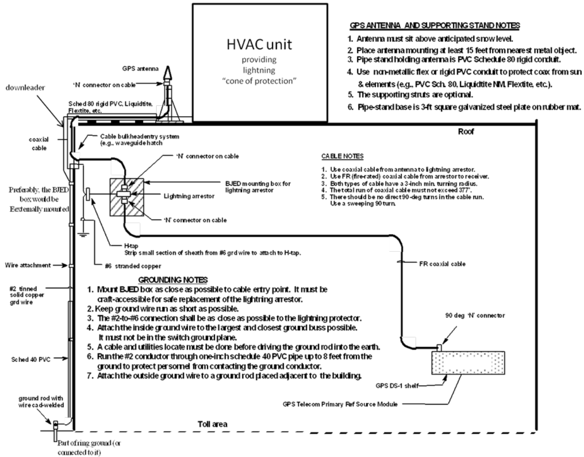
Figure 7-26: Rooftop GPS Antenna Grounding Detail
