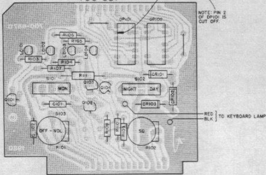
PARTS PLACEMENT CONTROL BOARD
