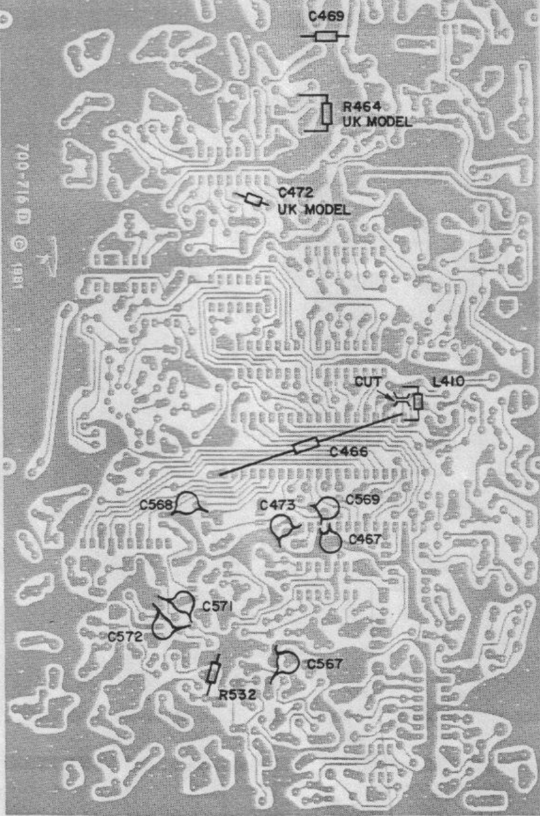
PARTS PLACEMENT BOTTOM SIDE
