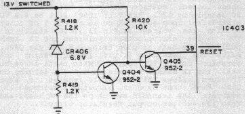
FIGURE 6 - RESET CIRCUIT WH2516
