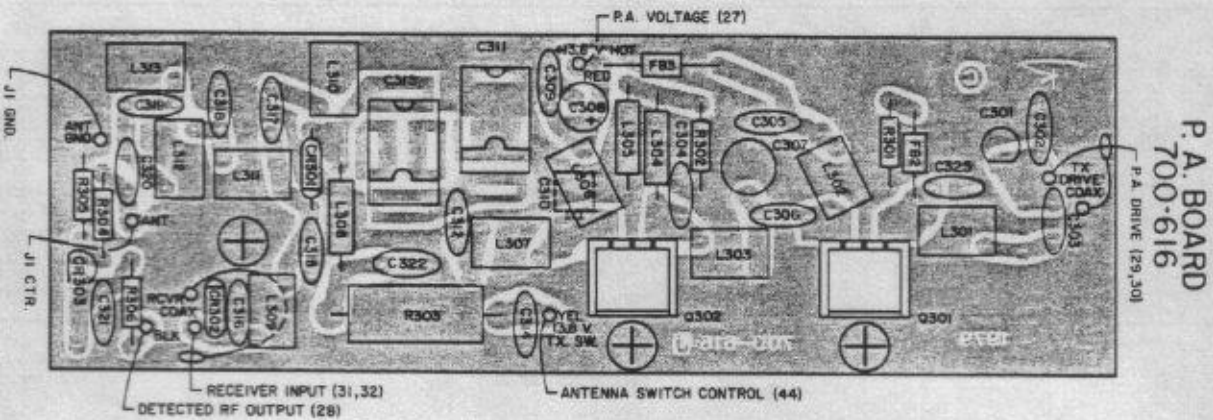
PARTS PLACEMENT P.A. BOARD
