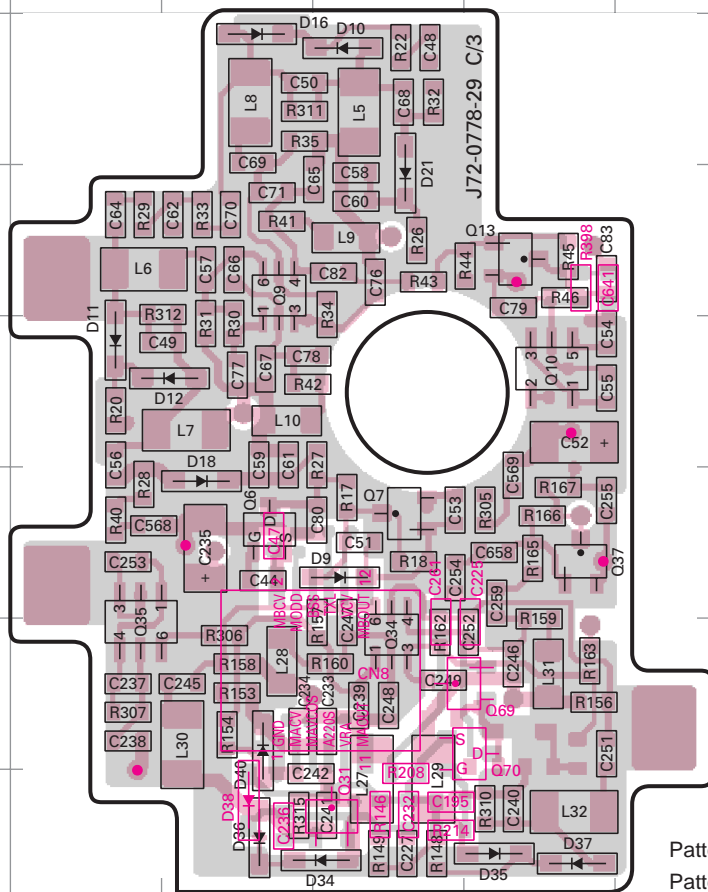
VCO SECTION(C/3) (Component side + Foil side)
