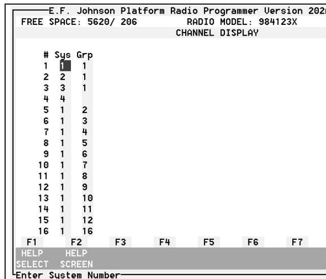
Figure 4-6 Channel Display Screen (Low Tier Only)
