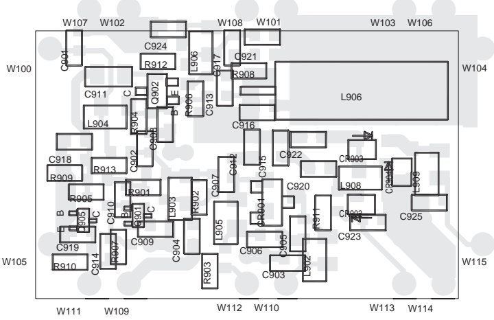
VCO BOARD LAYOUT (800/900 MHZ)
