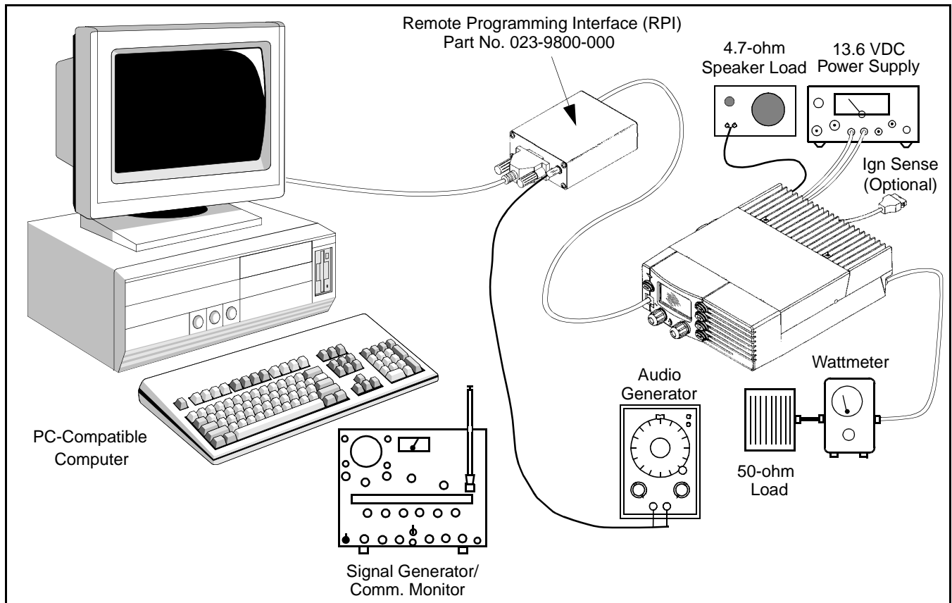
Figure 7-1 Alignment Setup
