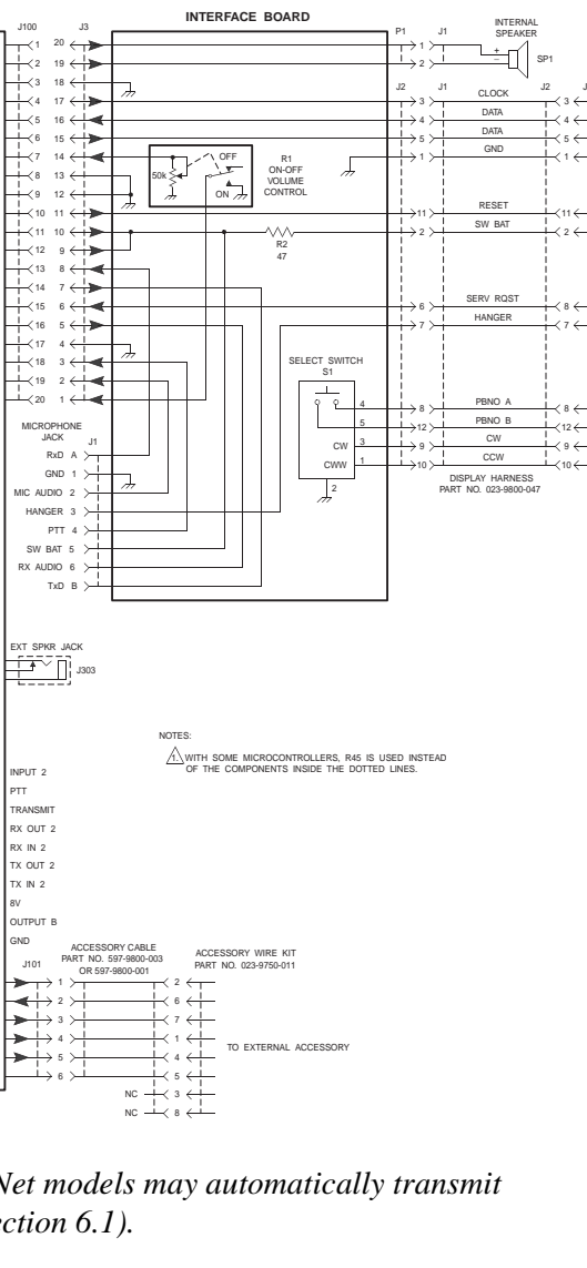
HIGH TIER INTERCONNECT SCHEMATIC
