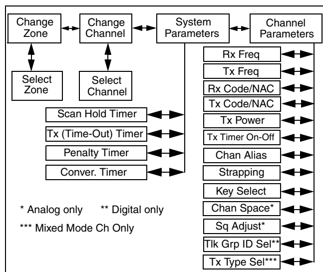
Figure 5-1 5300 Keypad Programming Menu Flowchart
