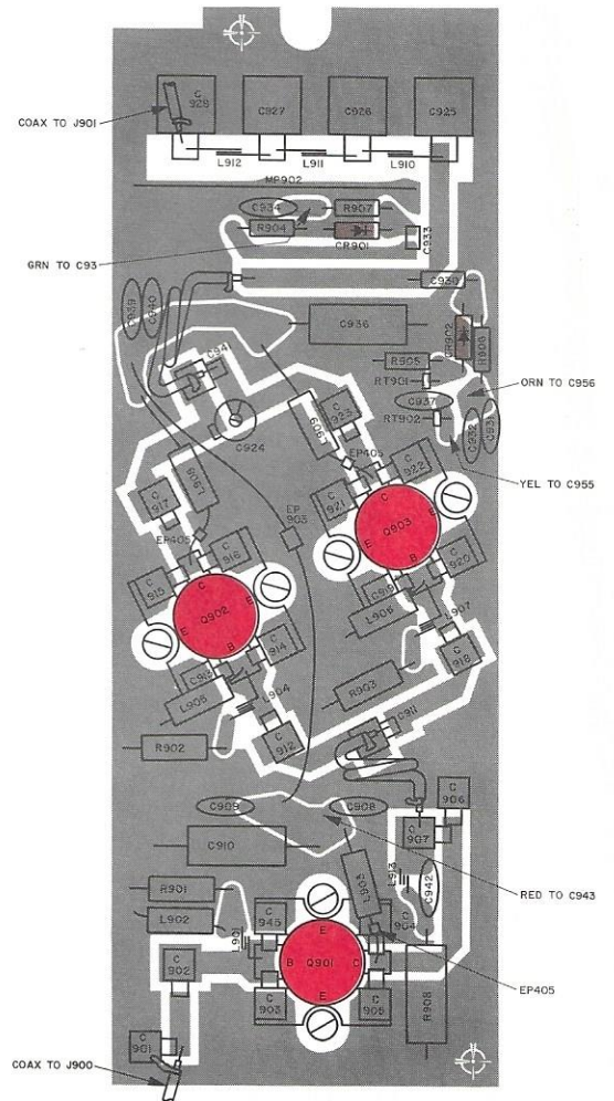
POWER AMPLIFIER BOARD COMPONENT LAYOUT (COMPONENT SIDE VIEW)
