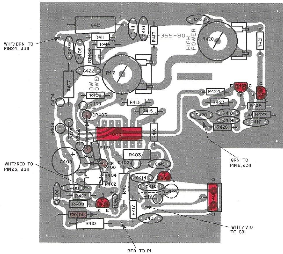
UNREVISED POWER CONTROL BOARD COMPONENT LAYOUT (SOLDER SIDE VIEW)
