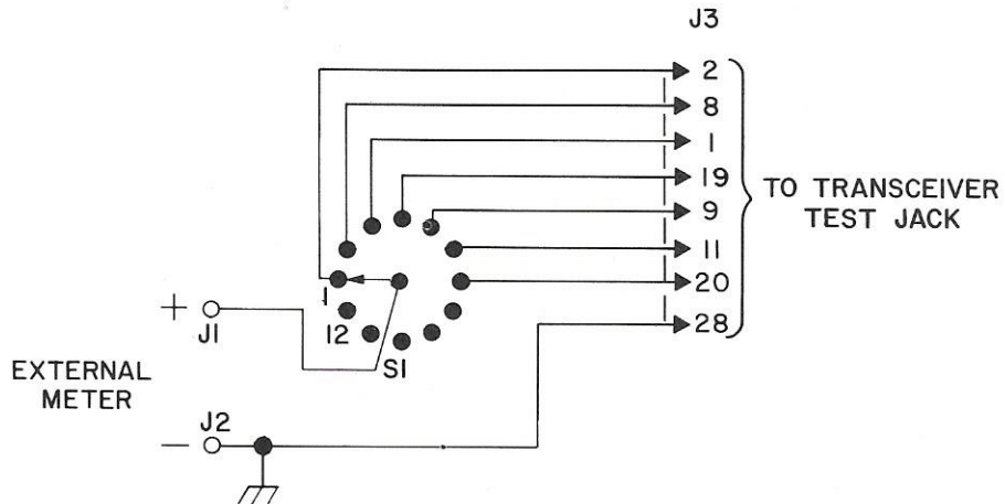
TEST PANEL SCHEMATIC DIAGRAM
