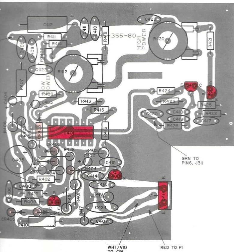
REVISED POWER CONTROL BOARD COMPONENT LAYOUT (SOLDER SIDE VIEW)
