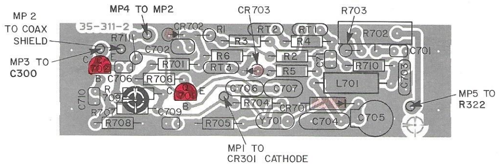
TCXO BOARD COMPONENT LAYOUT (SOLDER SIDE VIEW)
