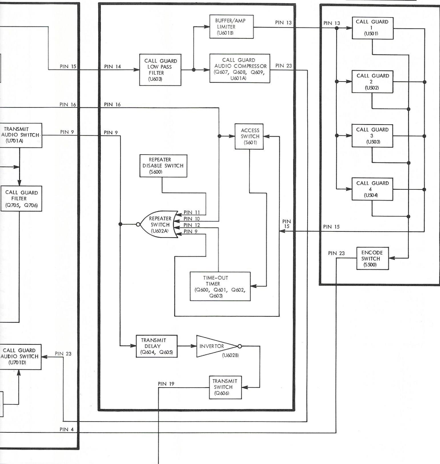
CARD RACK BLOCK DIAGRAM
