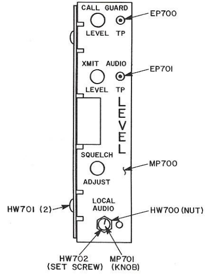
LEVEL ADJUST CARD FRONT PANEL
