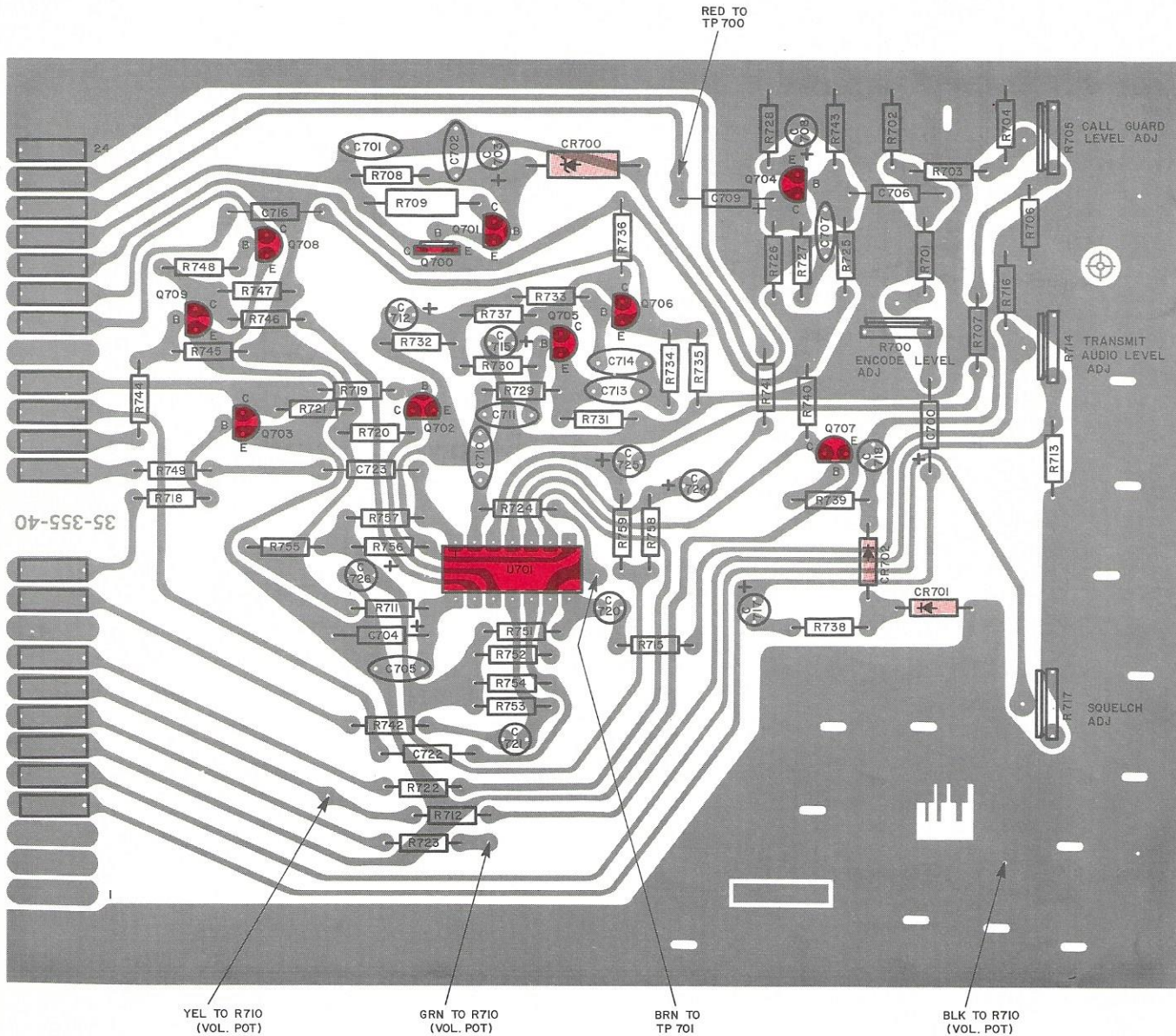
LEVEL ADJUST CARD COMPONENT LAYOUT (SOLDER SIDE VIEW)
