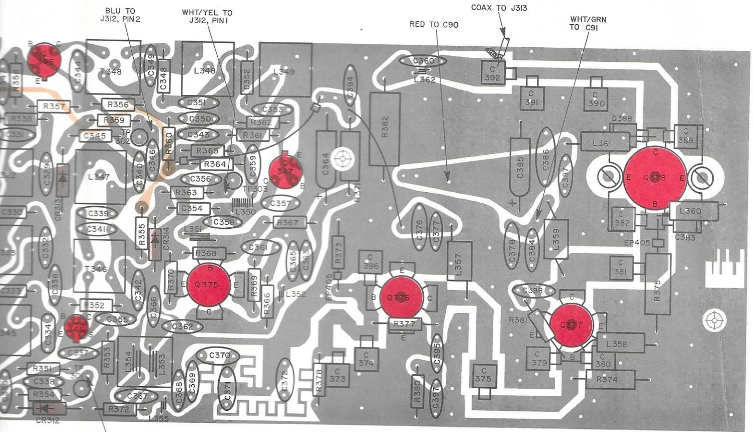
MP3 P2] WHT TO J312, PIN 8 CENTER BOARD COMPONENT LAYOUT (SOLDER SIDE VIEW)
