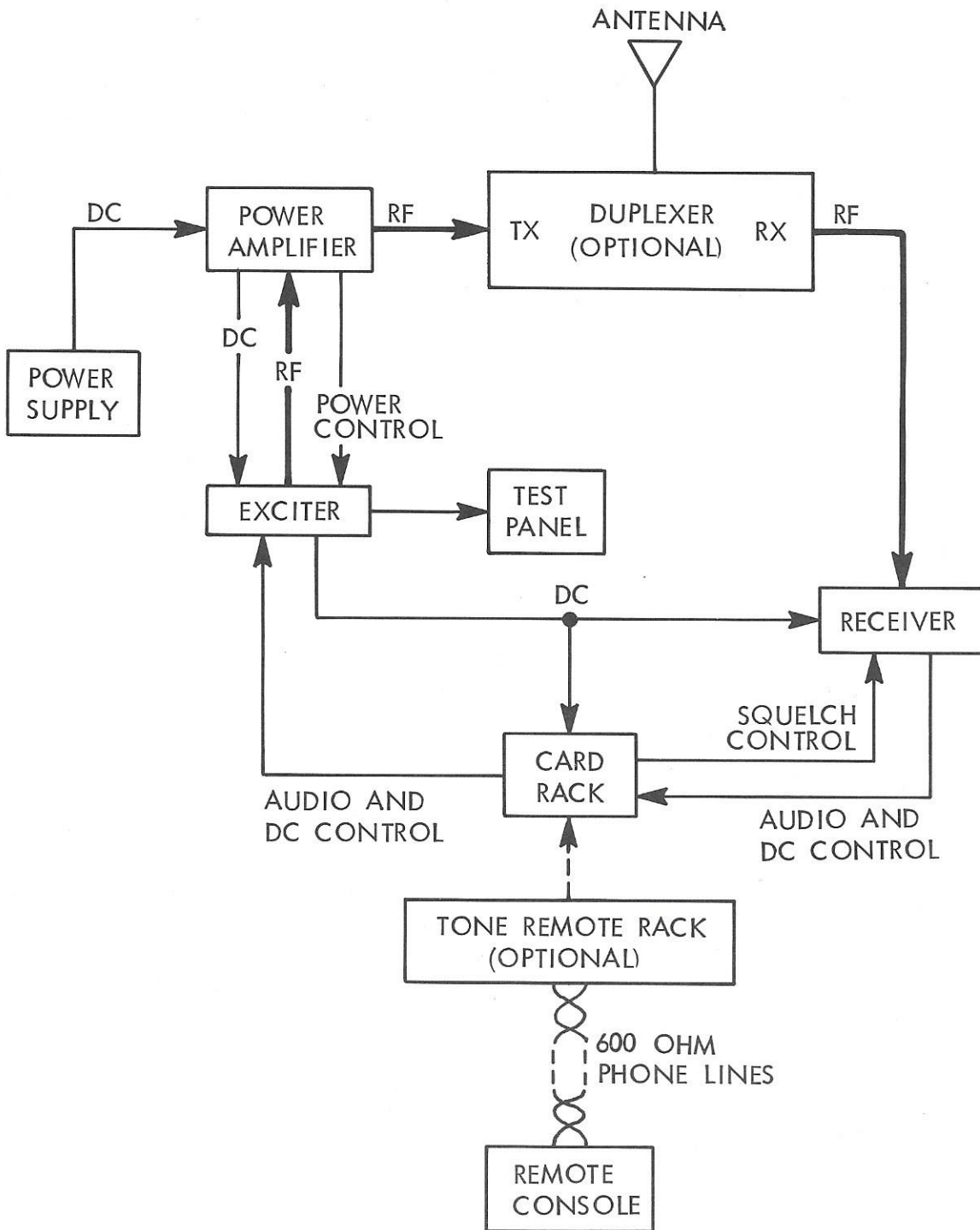
REPEATER BLOCK DIAGRAM
