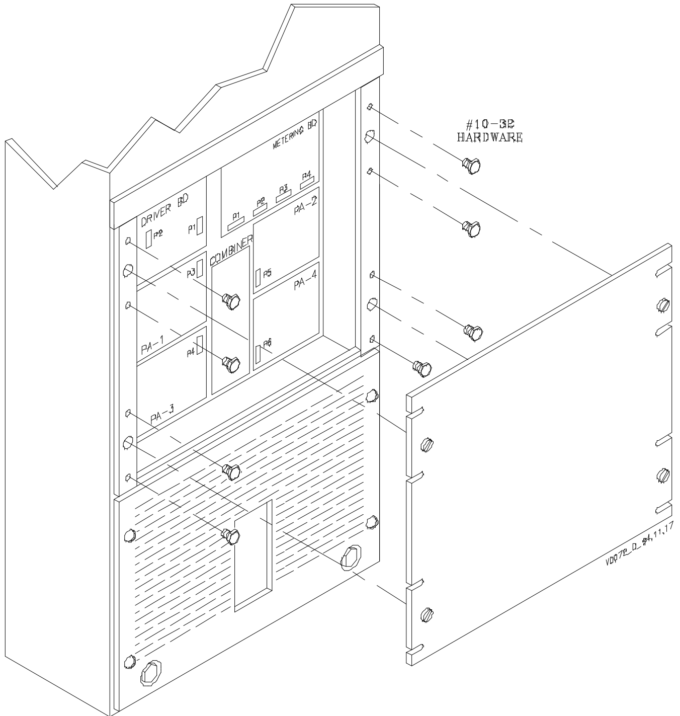
Figure 3-1 500-Watt, 900-MHz Power Amplifier Front View
