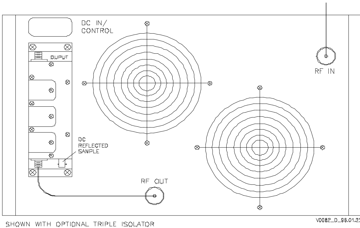
Figure 3-2 500-Watt, 900-MHz Power Amplifier Rear View
