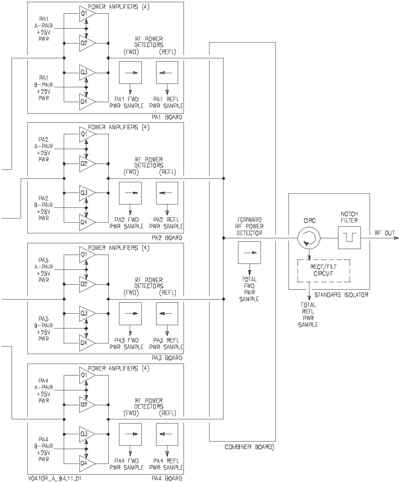
Figure 6-3 500-Watt PA Detailed Functional Diagram (continued)
