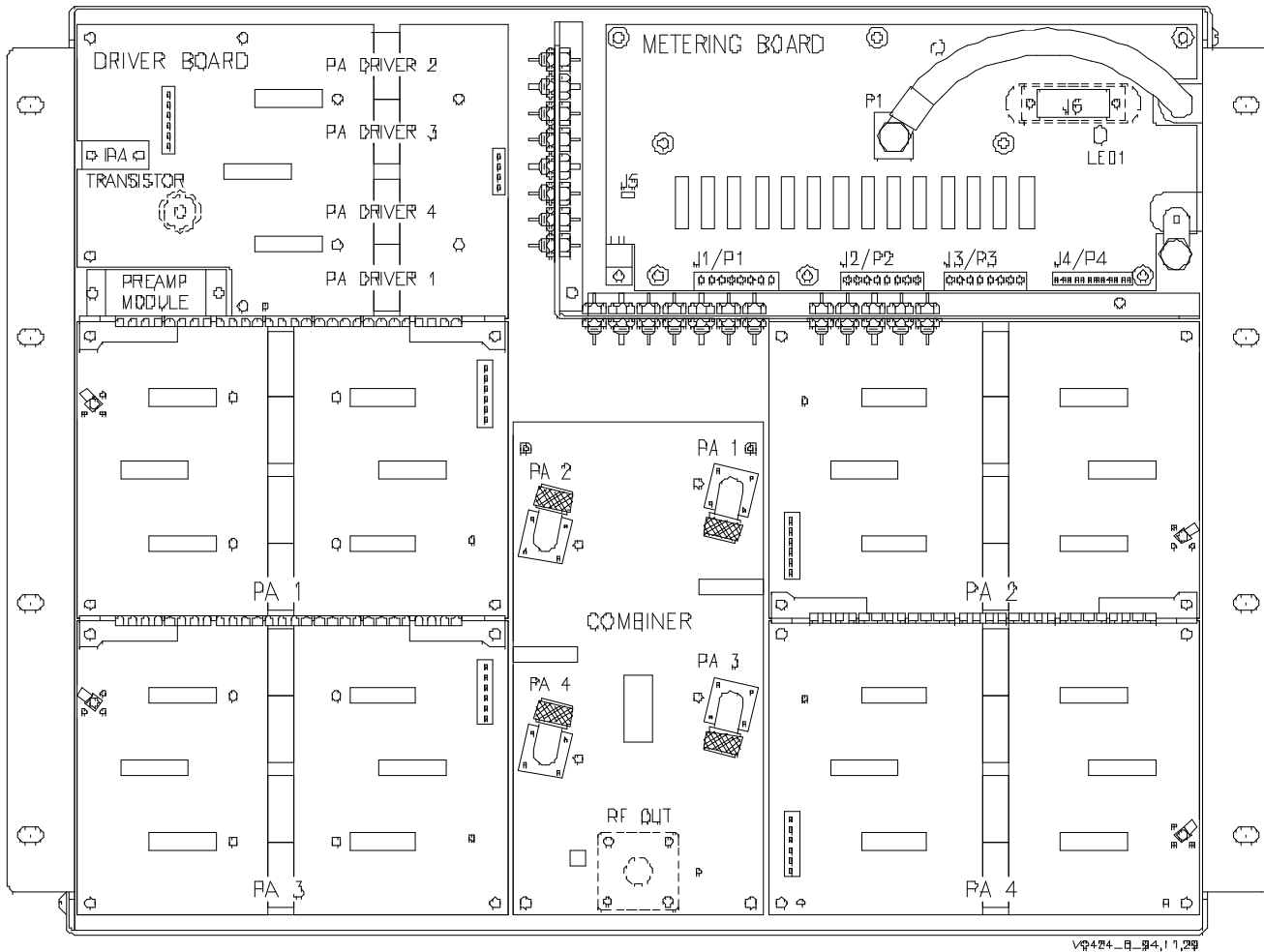
Figure 5-1 Front-Panel View with Cover Removed
