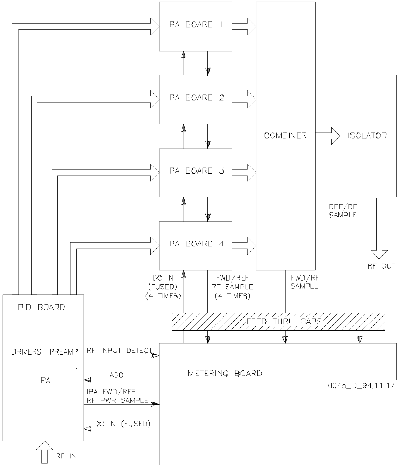
Figure 3-3 Simplified Block Diagram
