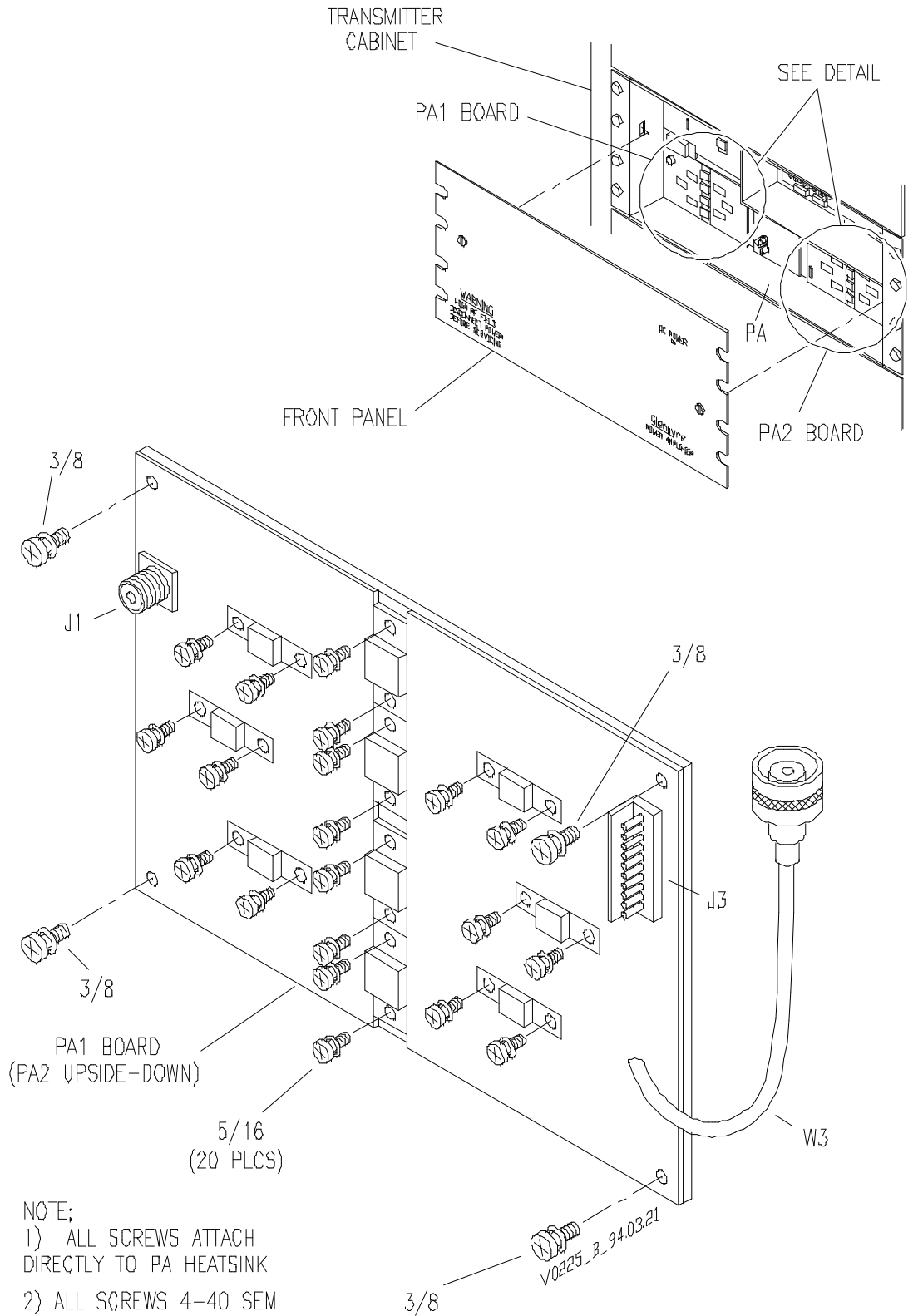
Figure 9-2 PA RF Module Removal and Reinstallation
