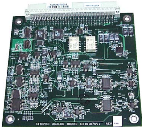
CB101070V1 Analog Filter Board
