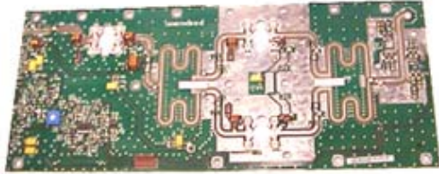
Power Amplifier Board(UHF) (Used in 19D902797 Series PA Assemblies)
