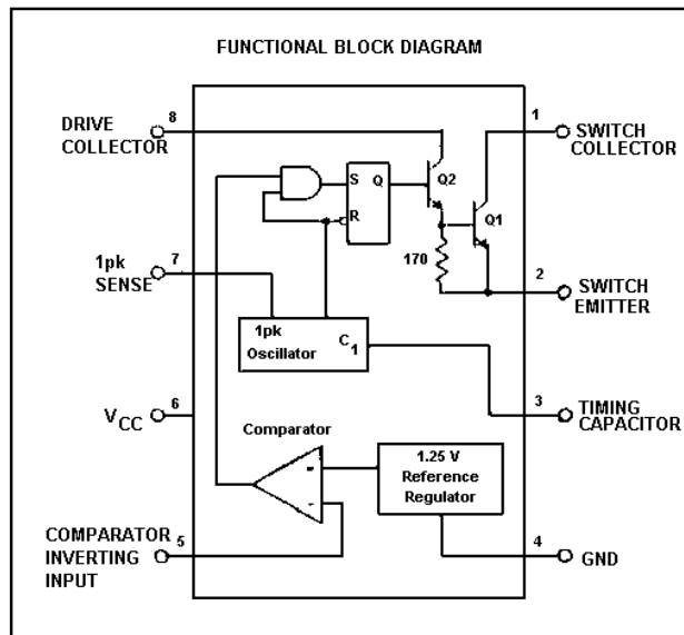
U1 -5 VOLT REGULATOR 19A704971P5
