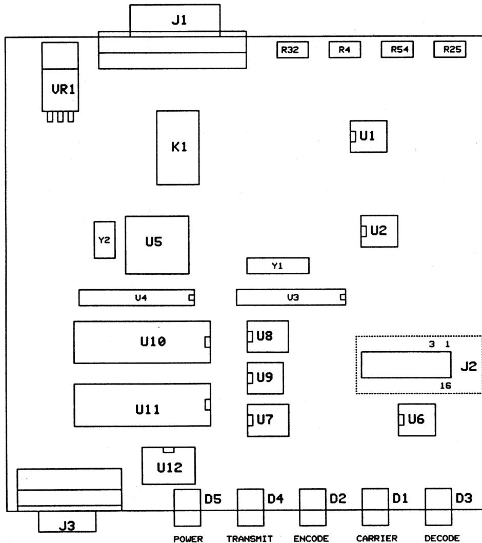
TP-3200 BOARD LAYOUT
