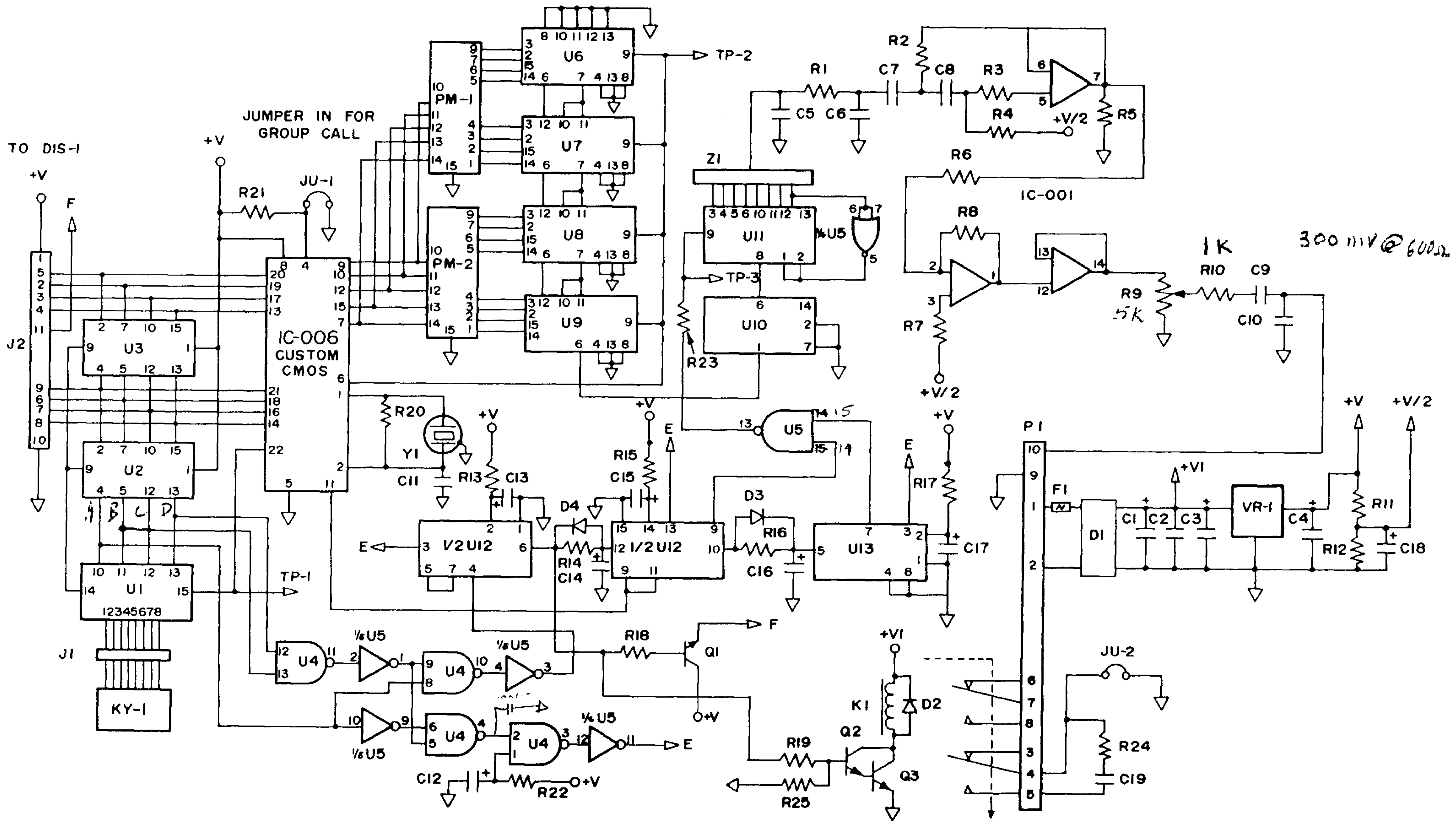
SCHMATIC DIAGRAM
