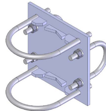
Clamp121C
