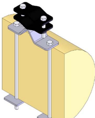
Clamp017B
