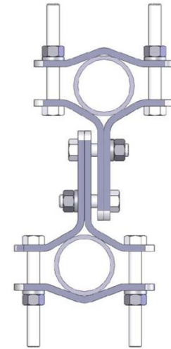
Clamp015
