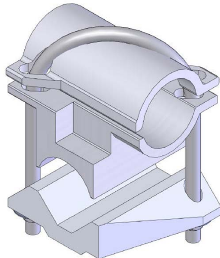
Clamp002B
