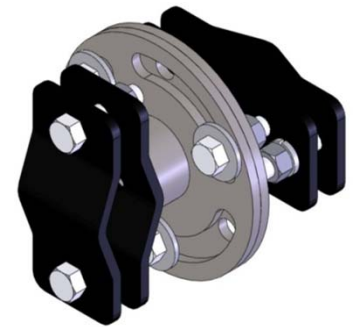
Clamp017H
