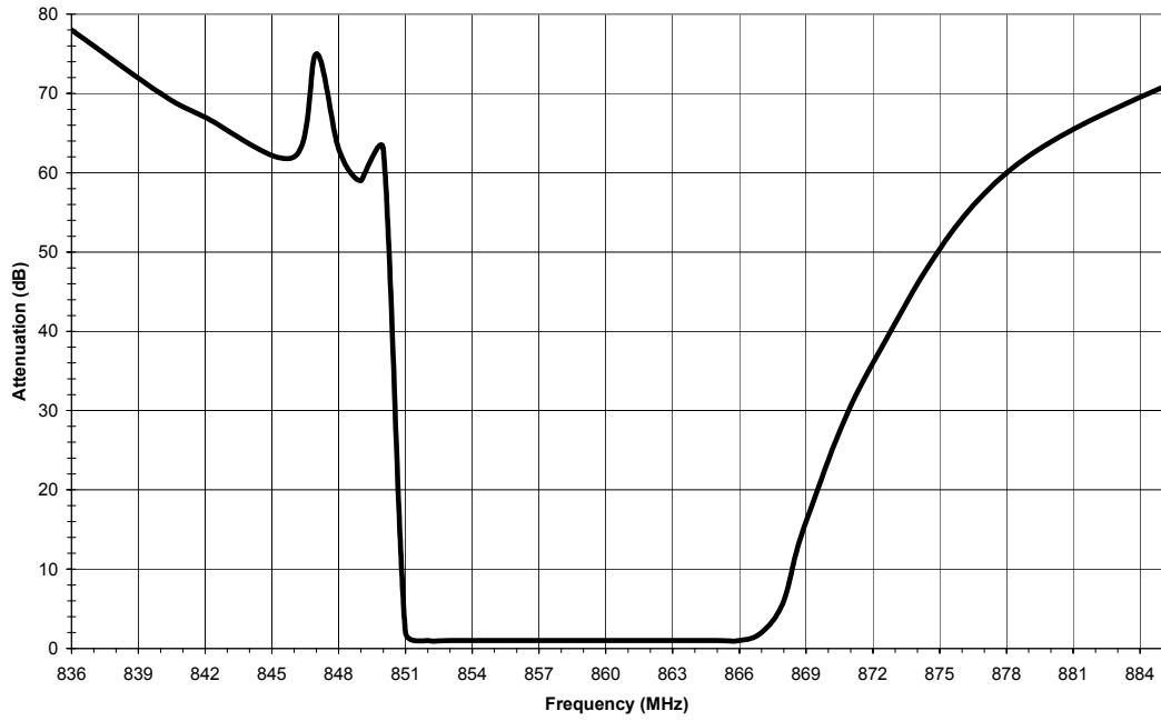
Figure 27 - Typical Motorola iDEN Base Station Internal Bandpass Filter
