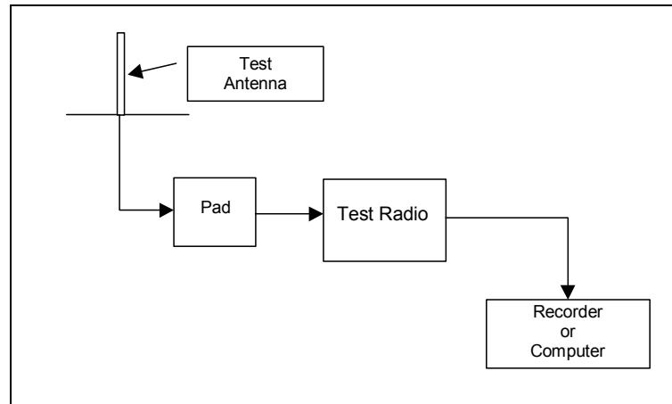
Figure 16 - Intermodulation Test
