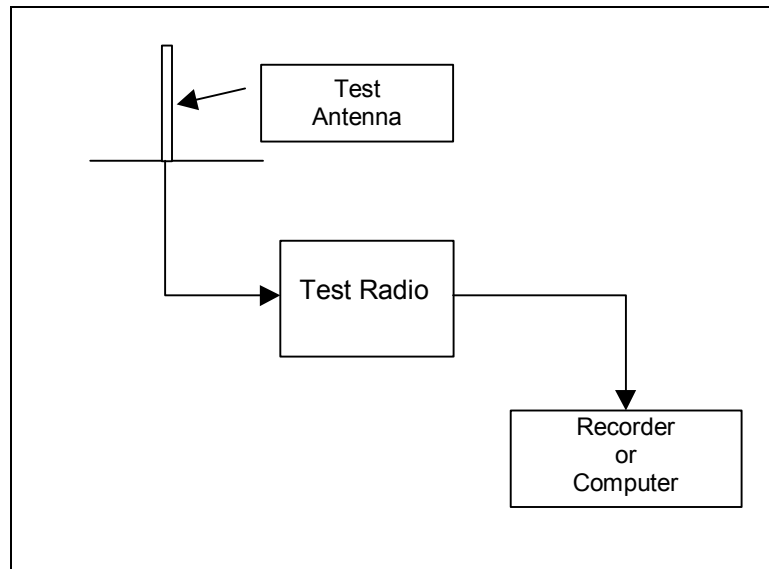
Figure 12 - Initial Evaluation
