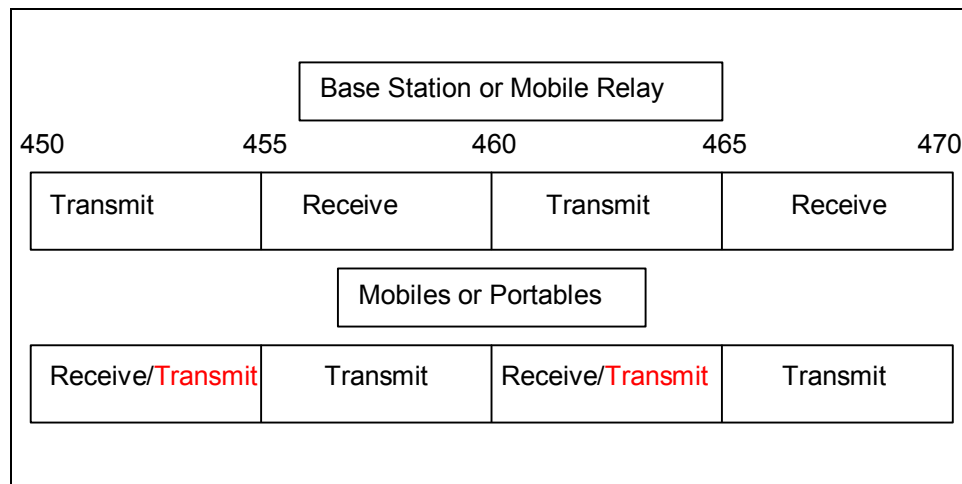
Figure 1 - 450 MHz Band
