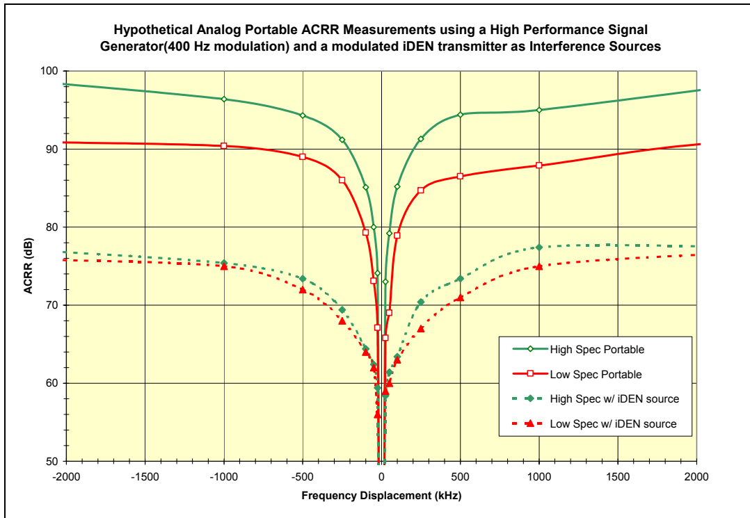
Figure 7 - Receiver Desensitization
