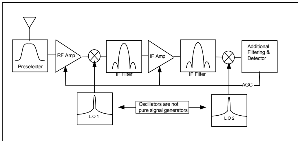
Figure 6 - Typical Receiver
