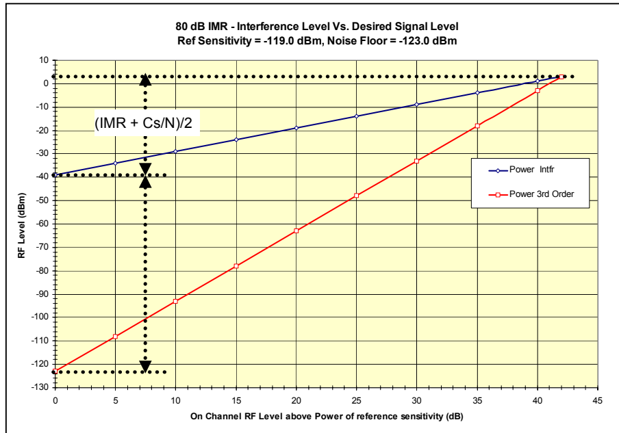
Figure 10 - IMR Performance
